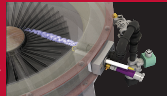
Patented Turbo Pilot 8,000 BTU/h Surefire Ignition System
